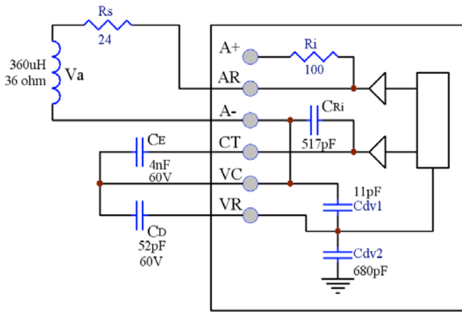
125kHz generic coil design.
