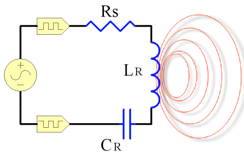
Figure 1. Basic tuned circuit
