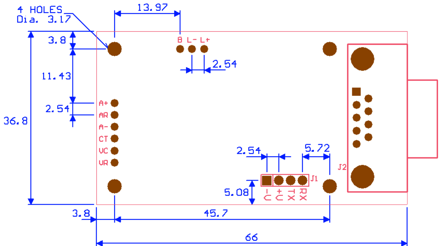
All dimensions in Millimeters.
